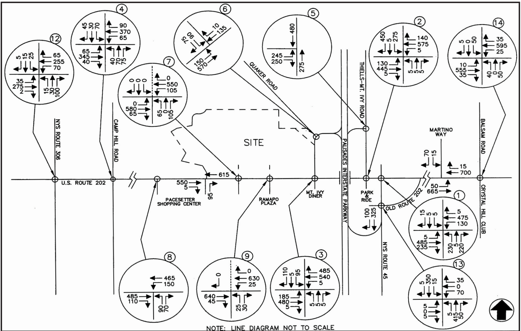
Figure 3.5-4: Existing Traffic Volumes Weekend Peak Saturday Highway Hour Minisceongo Park
